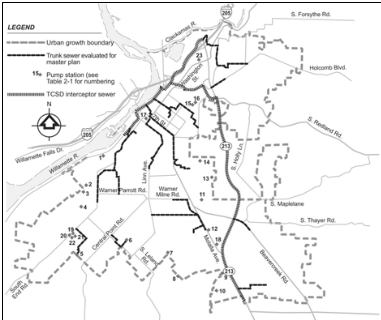
Figure 2-5. Existing Trunk Sewers and Pump Stations Evaluated for Master Plan
