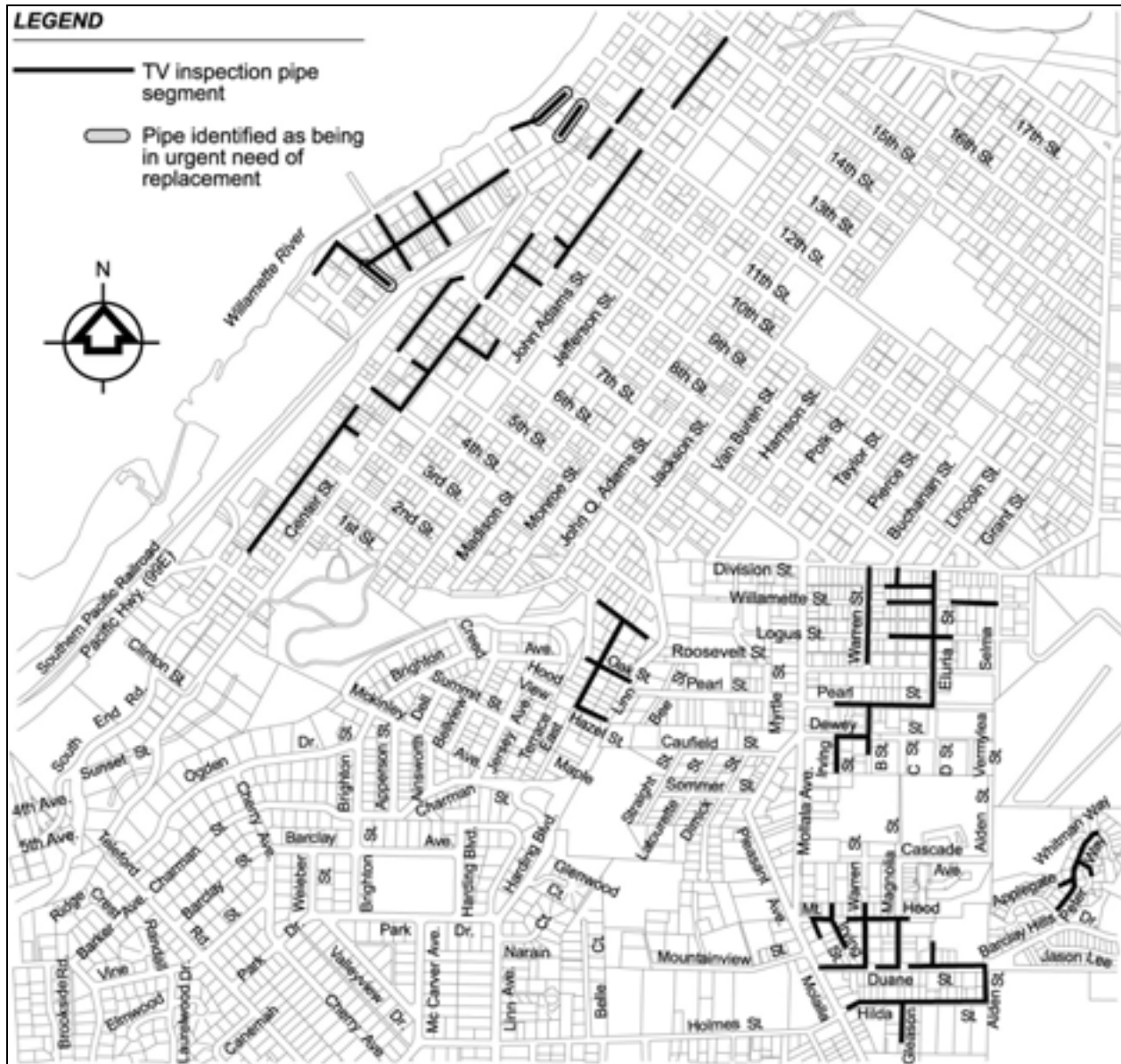
Figure 2-7. Extent of TV Sewer Inspection and Pipes in Urgent Need of Replacement
