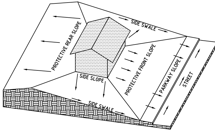
LOT GRADING TYPE B ALL DRAINAGE TO STREET AND REAR LOT LINE
